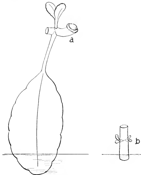
FIG. 84.—Influence of leaf on callus formation in stem. Stem a , with leaf, forms callus, while stem b , without leaf, does not during the same time. Nov. 15 to Dec. 12.
